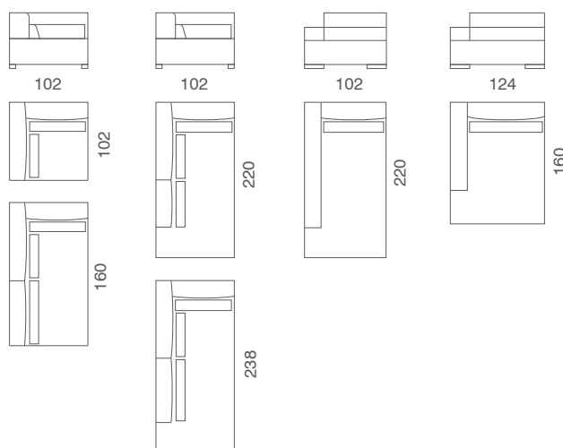
Chaise longue dx o sx Chaise longue with right or left short arm
